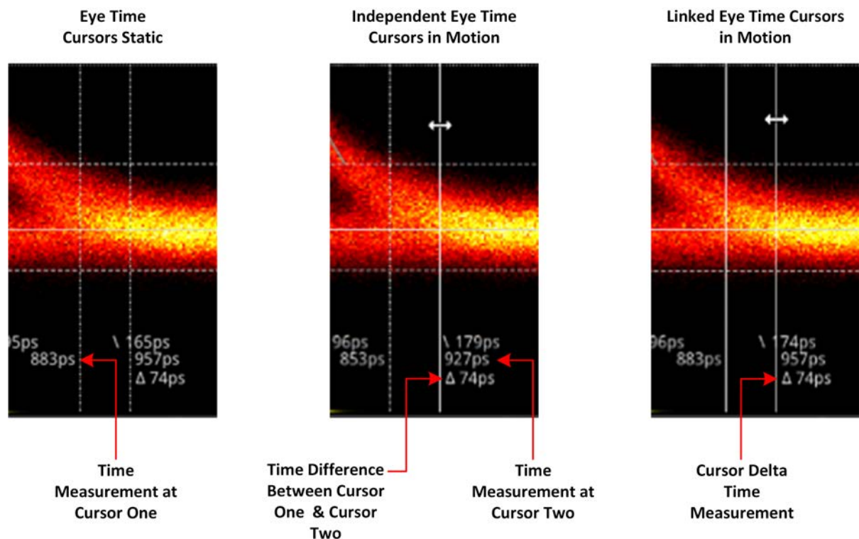
Figure 14-2: Advanced SDI Stress Option: Eye Time Cursors
