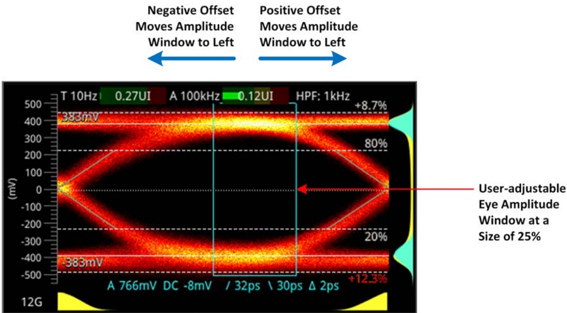
Figure 14-4: Advanced SDI Stress Option: Amplitude Window
