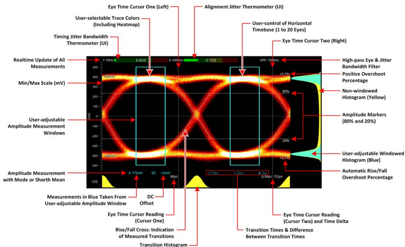
Figure 14-1: 12G-SDI Eye Pattern Display with 100 kHz Jitter Filter
