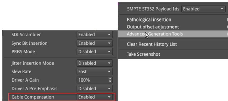
Figure 14-3: Advanced Generation Tools Option Menu
