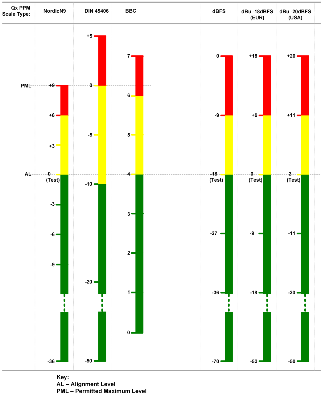
Figure 10-5: Comparison of Audio Metering Scales
