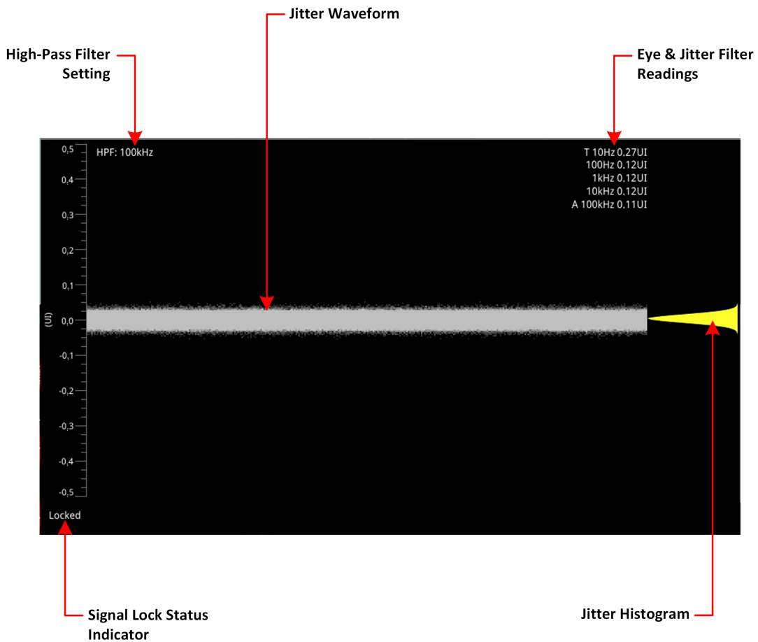
Figure 13-4: Jitter SDI In A Instrument
