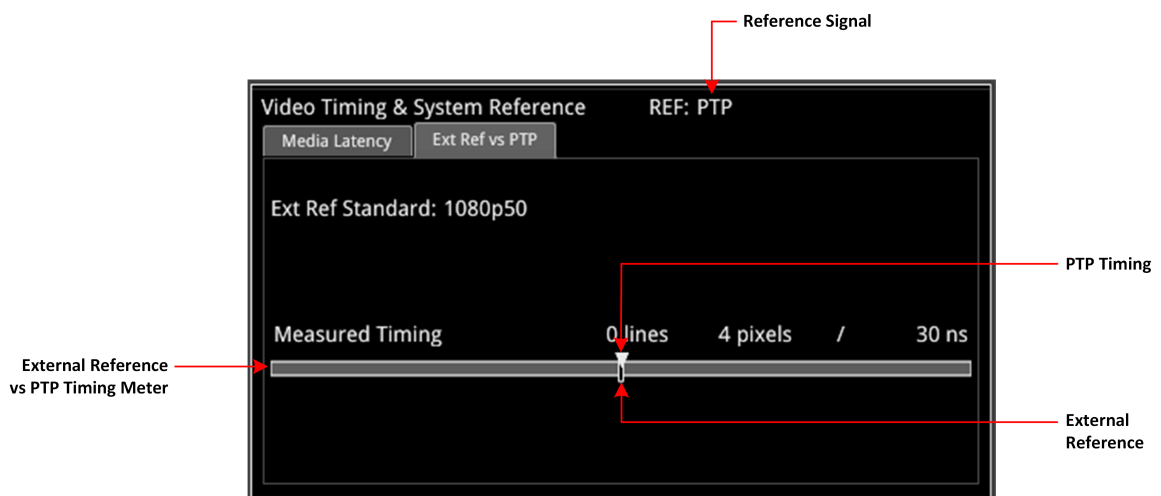
Figure 5-23: Ext Ref vs PTP Tab of the Video Timing & System Reference Instrument (IP 2110 Mode)
