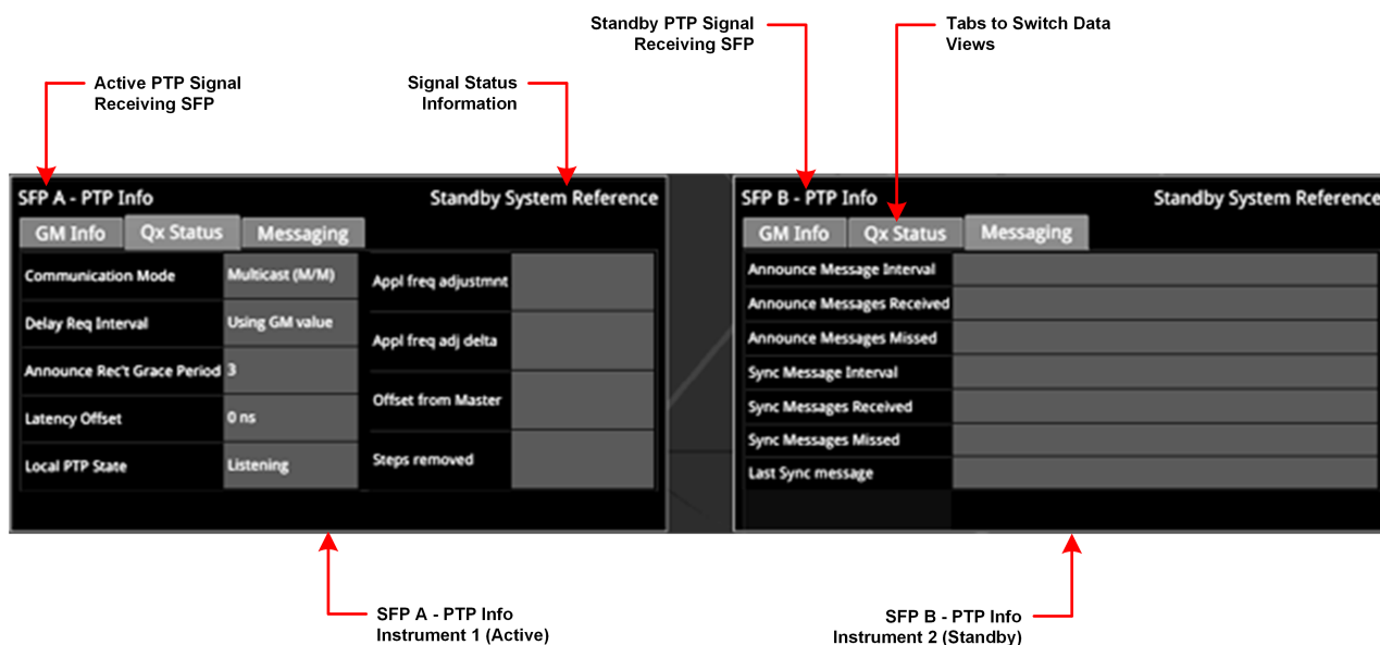
Figure 5-20: Dual SFP A and B - PTP Info Instruments (IP 2110 Mode)
