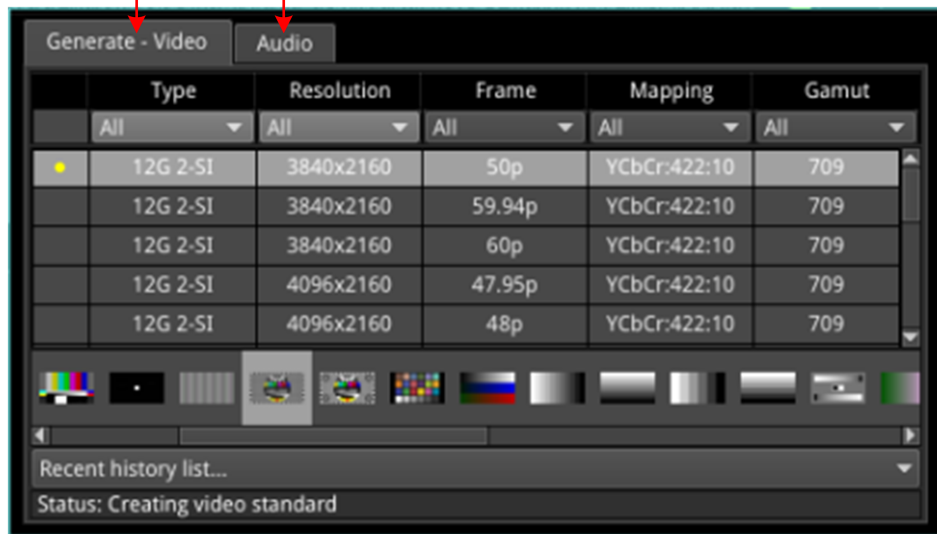
Figure 2-19: Example of Tabs in the Generator - Configuration Instrument
