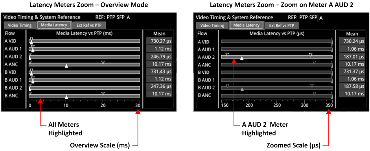
Figure 12-11: Media Latency Tab of the Video Timing & System Reference Instrument (IP 2110 Mode) Detailed information about the Media Latency measurement is provided in the Appendix "Advanced Media Timing Measurements" on page B-2.
