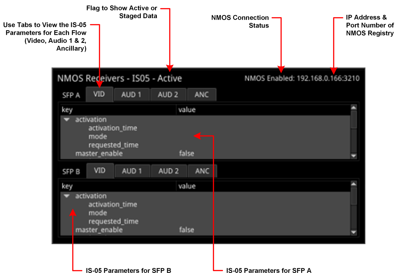
Figure 5-17: NMOS Receivers - IS05 Instrument (Single Interface, 1/16 Screen Size) (IP 2110 Mode)
