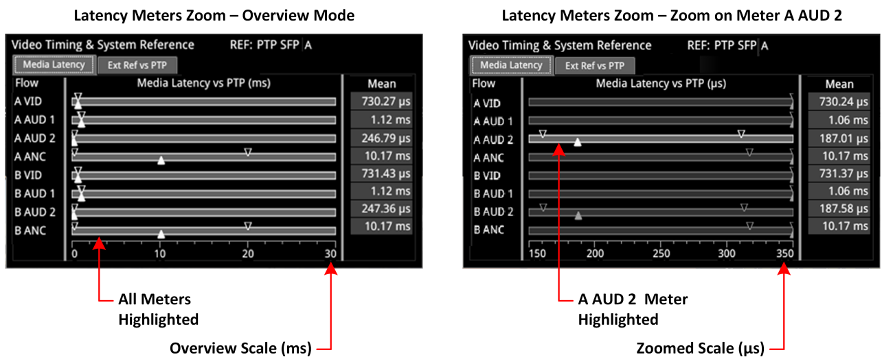
Figure 5-35: Media Latency Tab of the Video Timing & System Reference Instrument (IP 2110 Mode)
