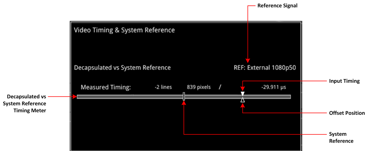
Figure 5-22: Video Timing & System Reference Instrument (IP 2022-6 Mode)
