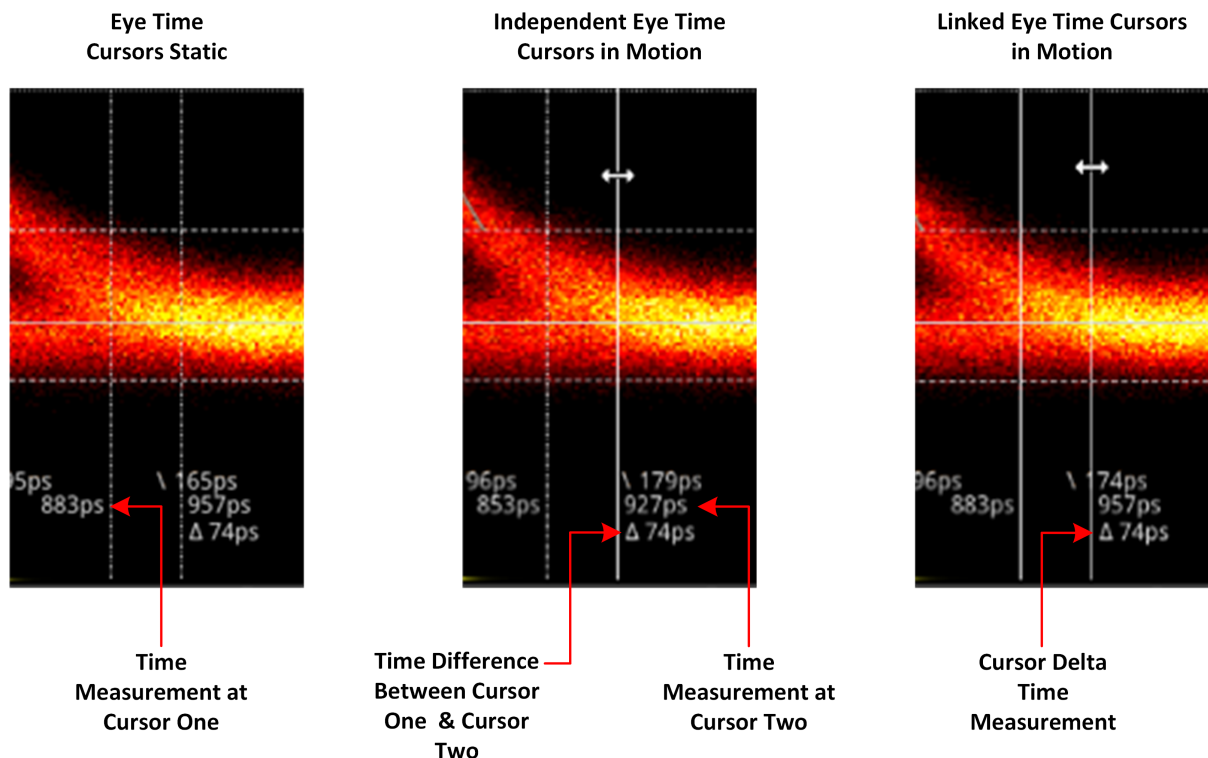
Figure 14-5: Advanced SDI Stress Option: Eye Time Cursors
