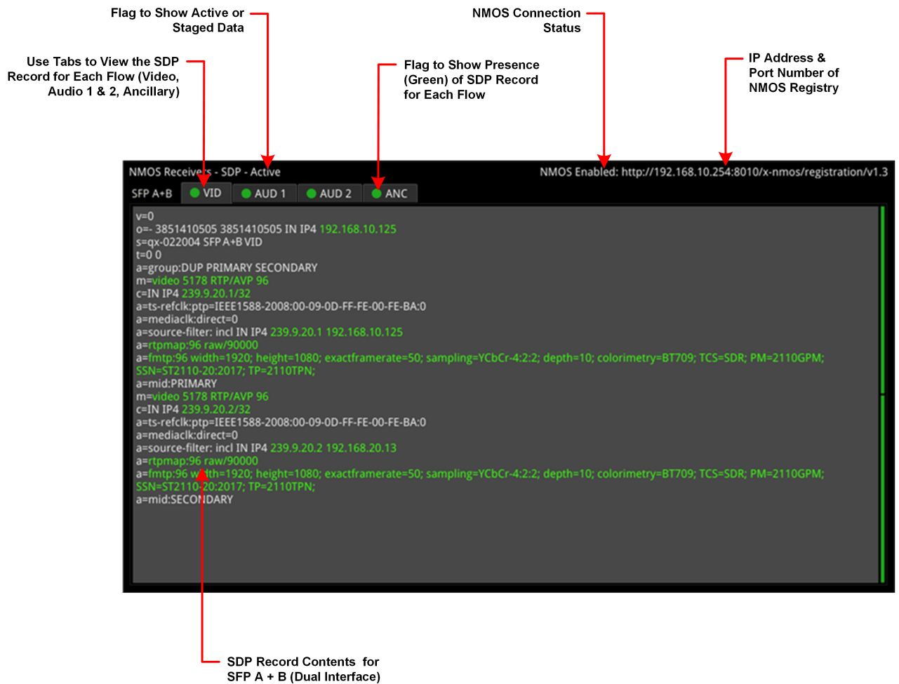
Figure 5-15: NMOS Receivers - SDP Instrument View (Dual Interface, 1/4 Screen Size) (IP 2110 Mode)
