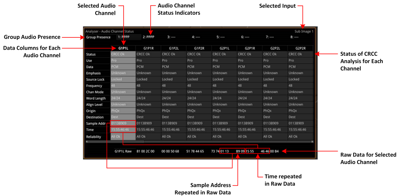
Figure 10-1: Analyzer - Audio Channel Status Instrument (SDI and ST 2022-6 Modes)
