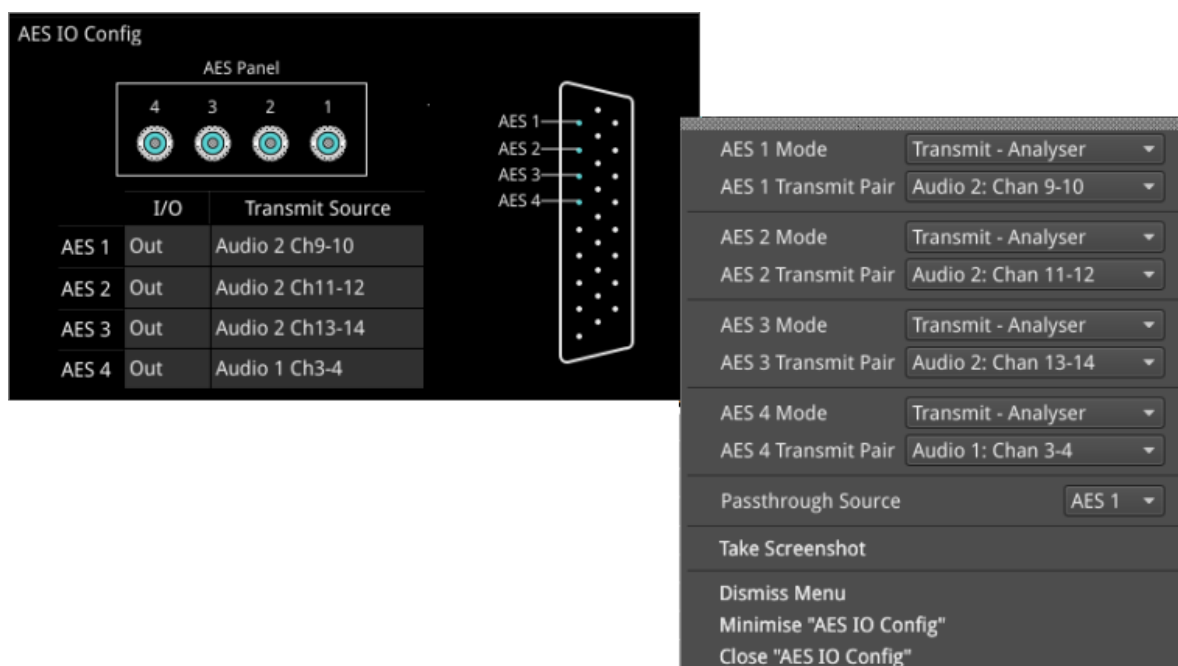
Figure 5-36: AES IO Config Instrument and Options Menu
