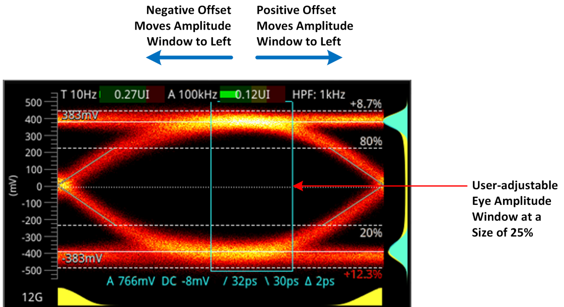
Figure 14-7: Advanced SDI Stress Option: Amplitude Window
