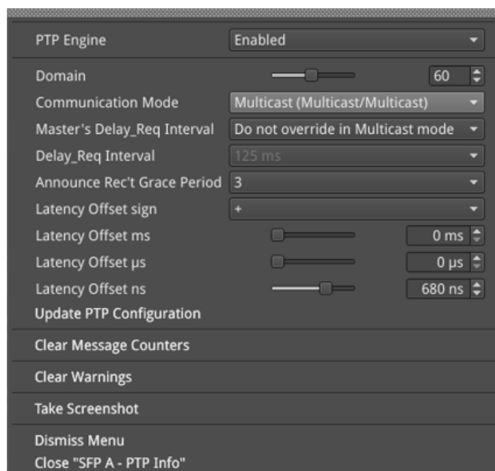
Figure 5-21: SFP A/B - PTP Info Instrument Menu Options
