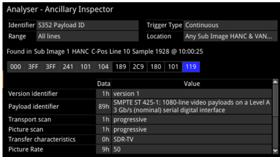
Figure 11-7: Analyzer - Ancillary Inspector Instrument (SDI and ST 2022-6 Modes)
