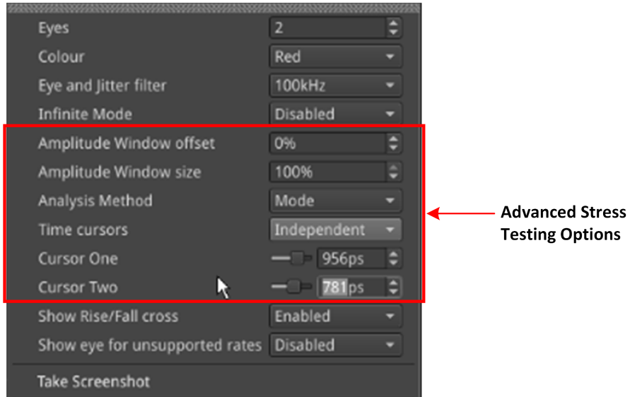
Figure 14-6: Eye - SDI In A Menu Showing Advanced Stress Testing Options
