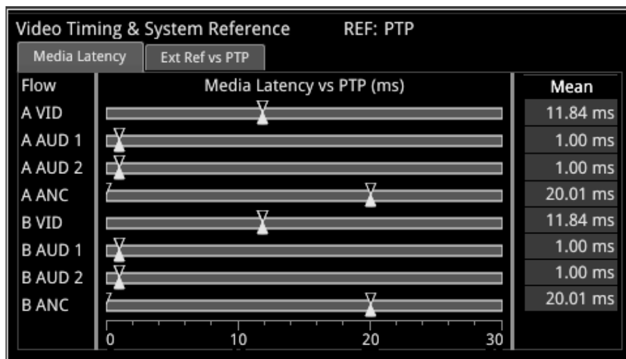
Figure 5-34: Media Latency Tab of the Video Timing & System Reference Instrument (IP 2110 Mode)
