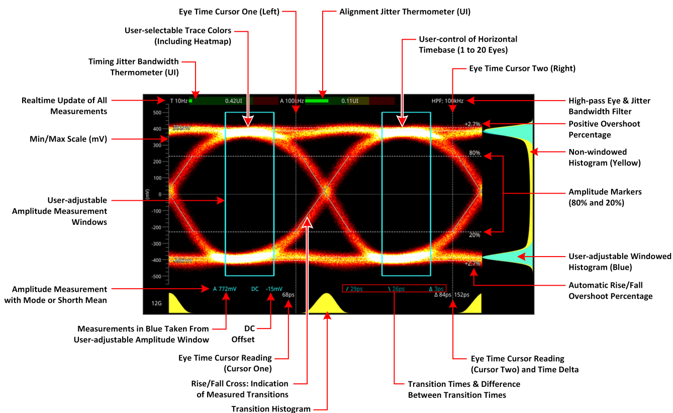
Figure 14-4: 12G-SDI Eye Pattern Display with 100 kHz Jitter Filter
