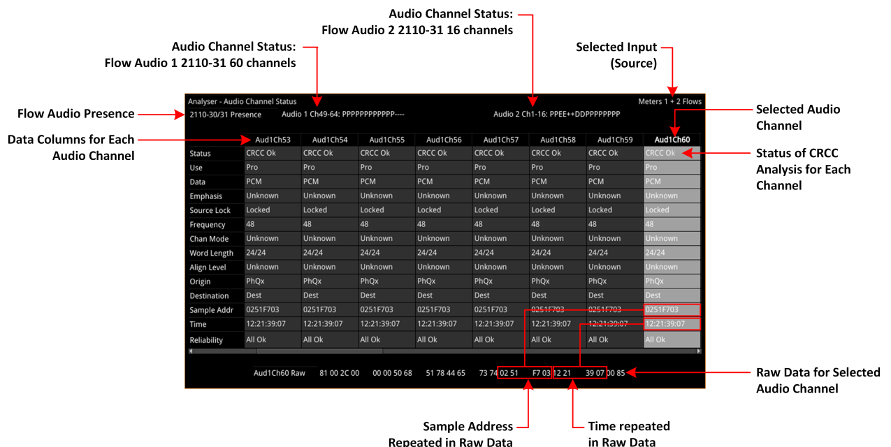
Figure 10-2: Analyzer - Audio Channel Status Instrument (ST 2110 Mode)
