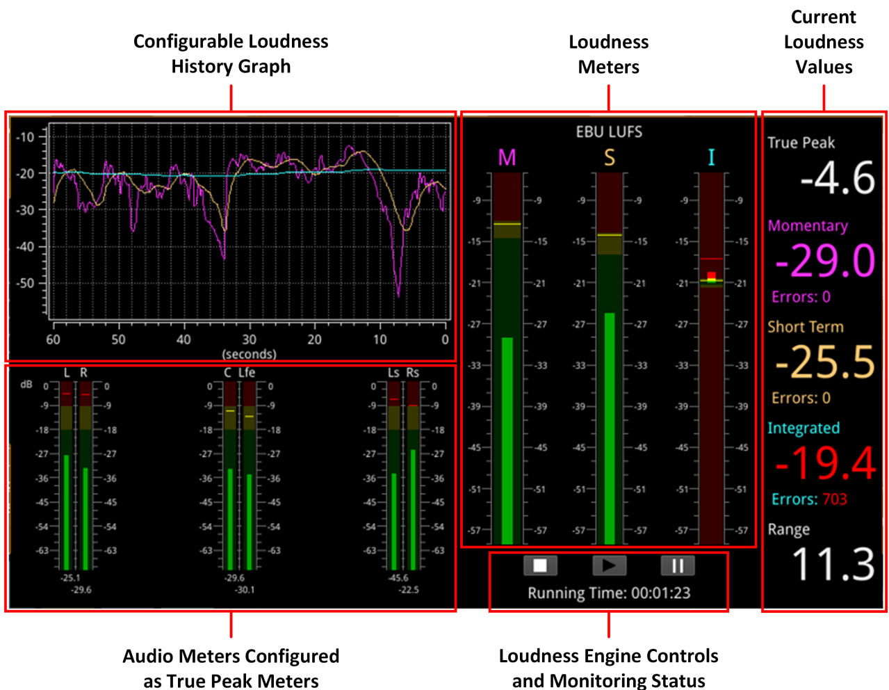
Figure 10-6: Analyzer - Loudness Monitor Instrument
