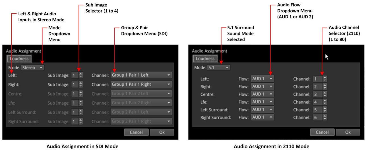
Figure 10-7: Audio Assignment for Loudness Input in SDI and 2110 Modes
