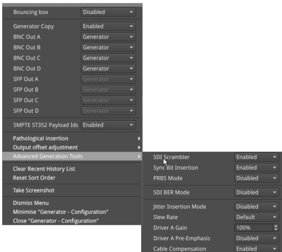
Figure 14-1: Advanced Generation Tools Option Menu
