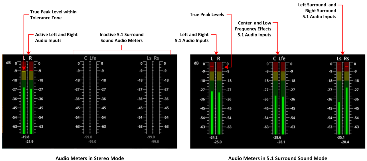
Figure 10-8: Audio Meters for Loudness Inputs in Stereo and 5.1 Surround Sound Modes
