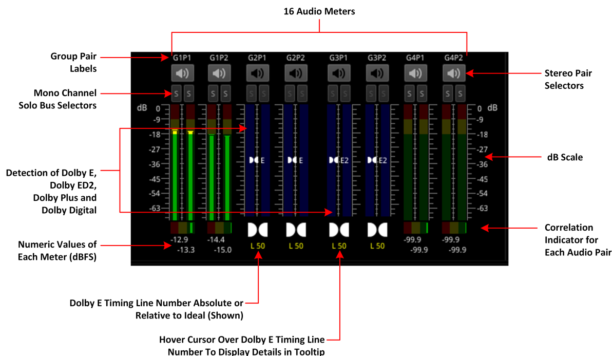
Figure 10-4: Analyzer - Audio Meters Instrument (SDI and 2022-6 Modes)
