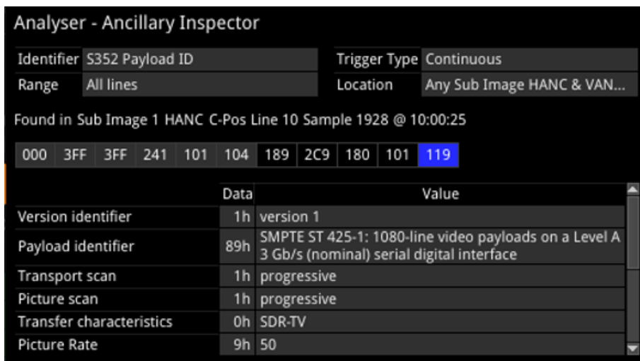
Figure 11-7: Analyzer - Ancillary Inspector Instrument (SDI and ST 2022-6 Modes)
