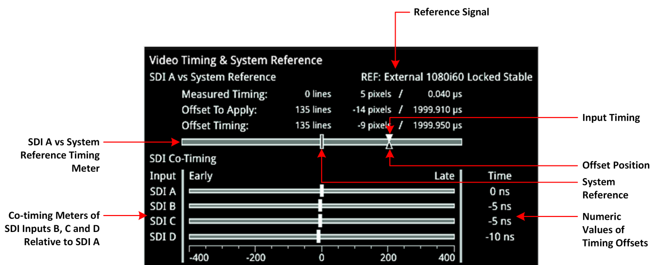
Figure 5-13: Video Timing & System Reference Instrument (SDI Mode)
