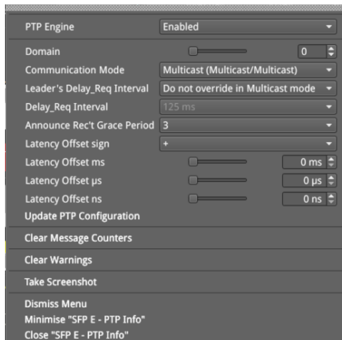
Figure 4-13: SFP E/F - PTP Info Instrument Menu Options
