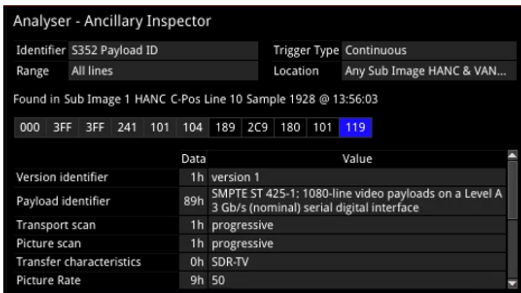
Figure 6-8: Analyzer - Ancillary Inspector Showing SMPTE ST352 Payload IDs
