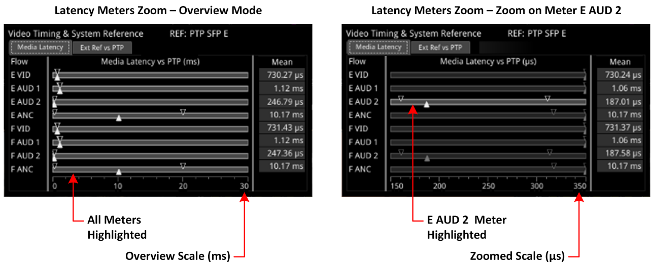
Figure 4-26: Media Latency Tab of the Video Timing & System Reference Instrument (IP 2110 Mode)
