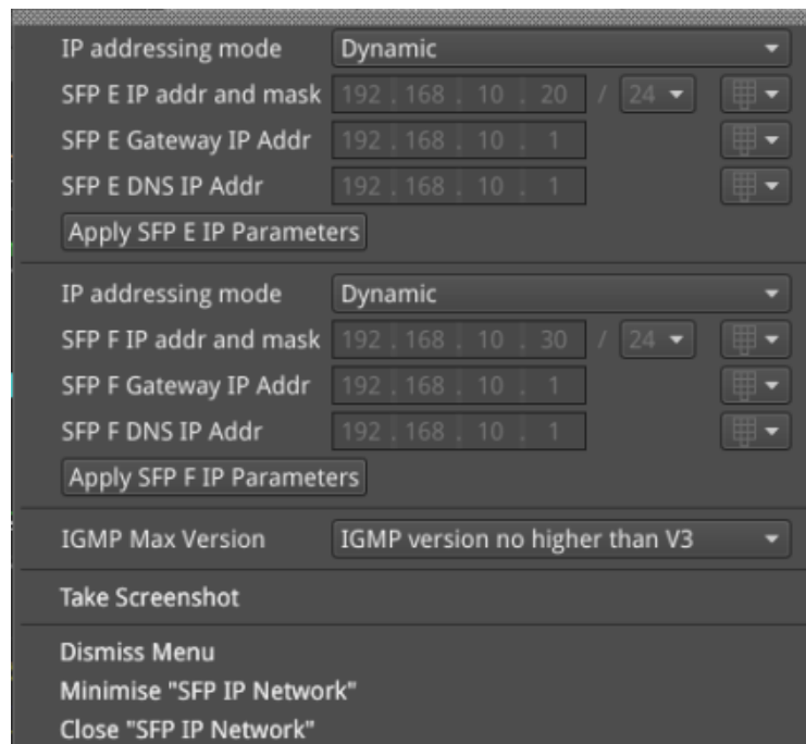
Figure 4-6: SFP IP Network Menu Options
