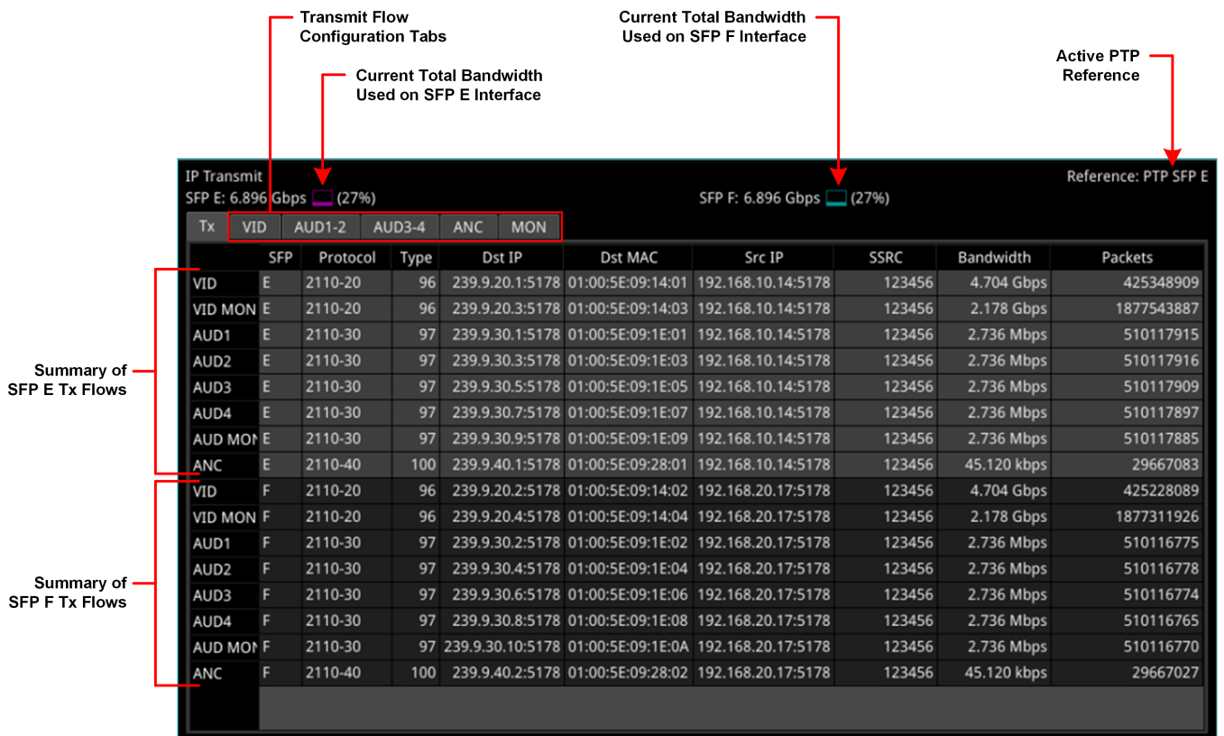
Figure 6-16: IP Transmit - Tx Tab (IP ST 2110 Mode)
