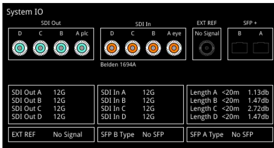
Figure 5-8: System IO Instrument Showing All 12G SDI Out and SDI In BNC Connectors In Use
