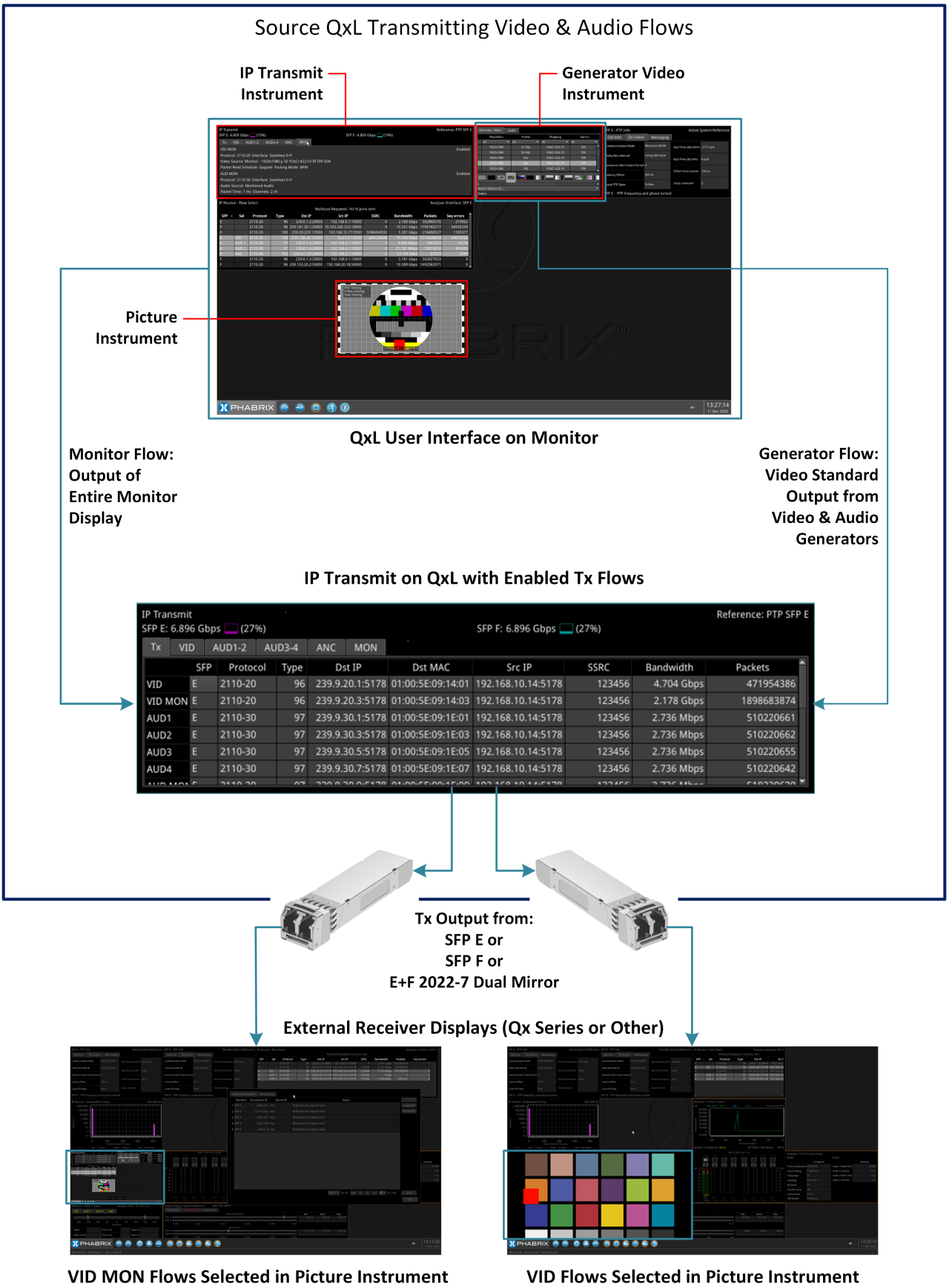
Figure 6-21: Schematic Overview of Transmission of Generator and Monitor Flows by the IP Transmit Instrument
