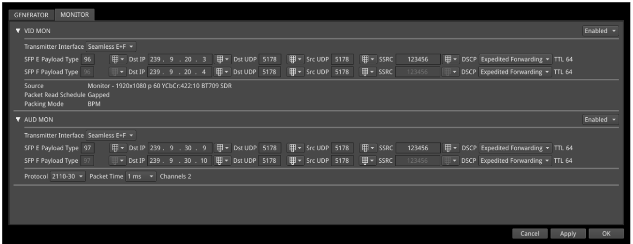
Figure 6-26: IP Transmit - MONITOR Video and Audio Flows Configuration
