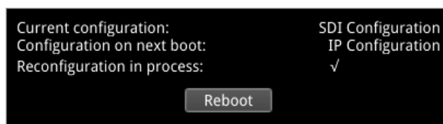
Figure 3-18: Reconfiguration Dialog
