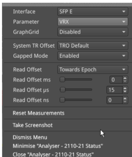
Figure 12-8: Analyzer - 2110-21 Status Menu Options for the VRX Parameter
