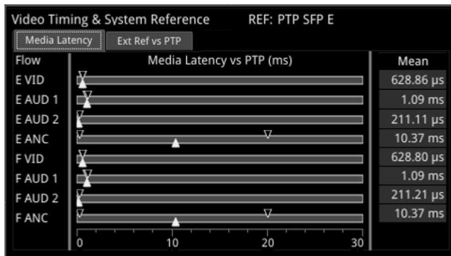
Figure 4-25: Media Latency Tab of the Video Timing & System Reference Instrument (IP 2110 Mode)
