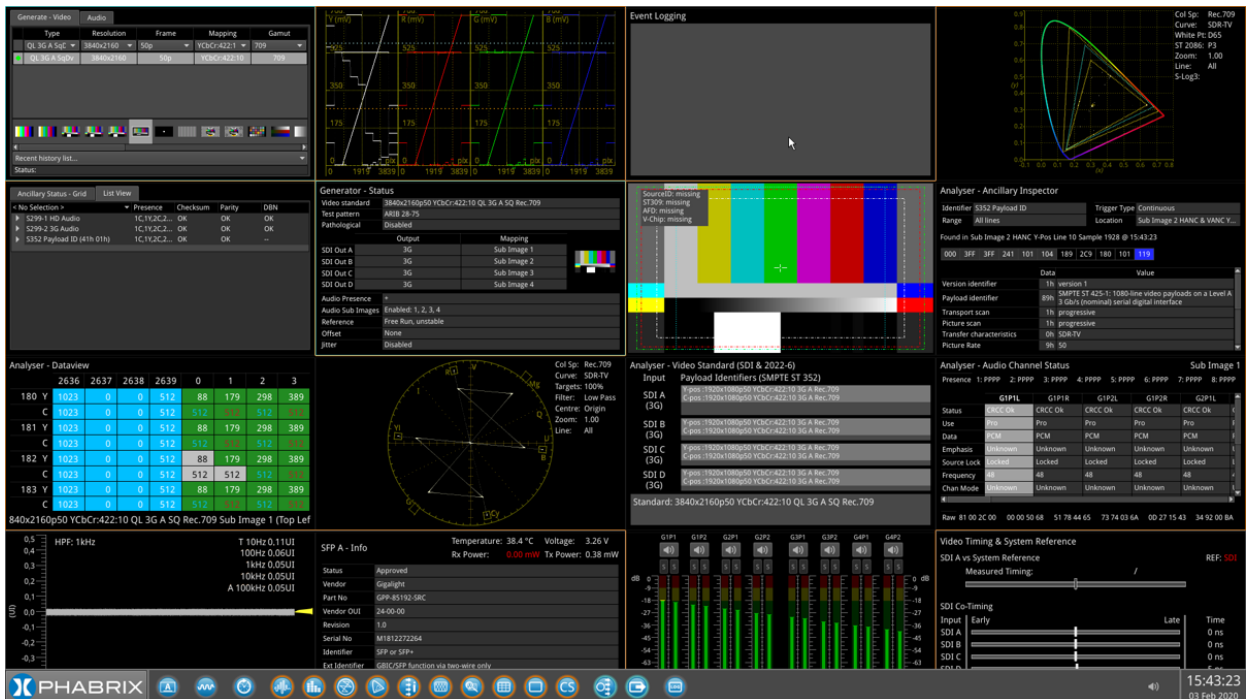
Figure 2-13: Full Screen with Active Instruments
