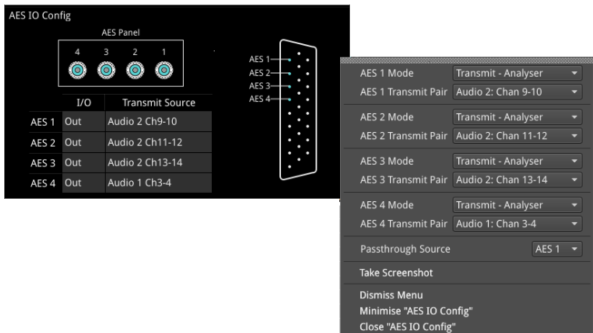
Figure 5-12: AES IO Config Instrument and Options Menu
